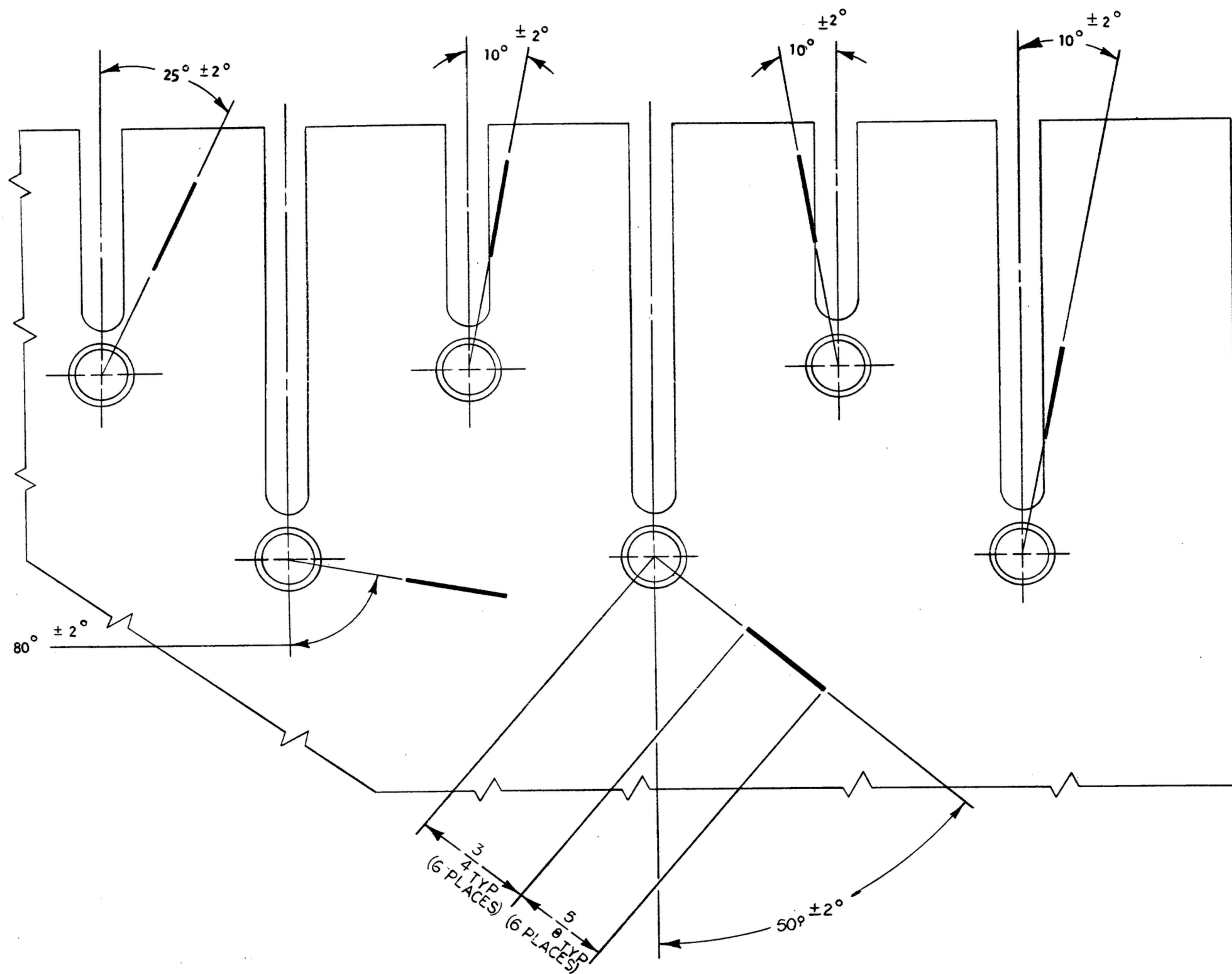
SILK SCREENING VIEW
