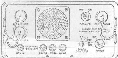
Figure 12. Radio Receiver R-121/URR, front panel.
